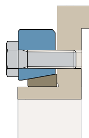
Half Shrink Disc Type HC
