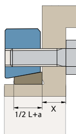
Half Shrink Disc Type HT
