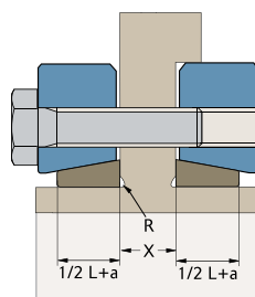
Split Shrink Disc
