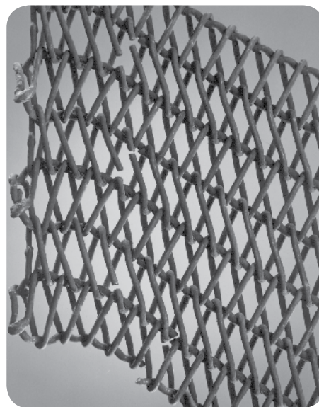
A damaged Double Balanced weave belt after five months of use. Note the camber and broken wires.
