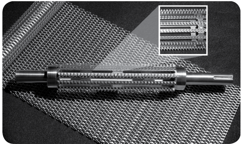
Patented self-cleaning hollow rolls are designed to make sanitation a breeze. Perfect for areas plagued by sanitation issues and applications prone to buildup. U.S. patent #7,565,967
